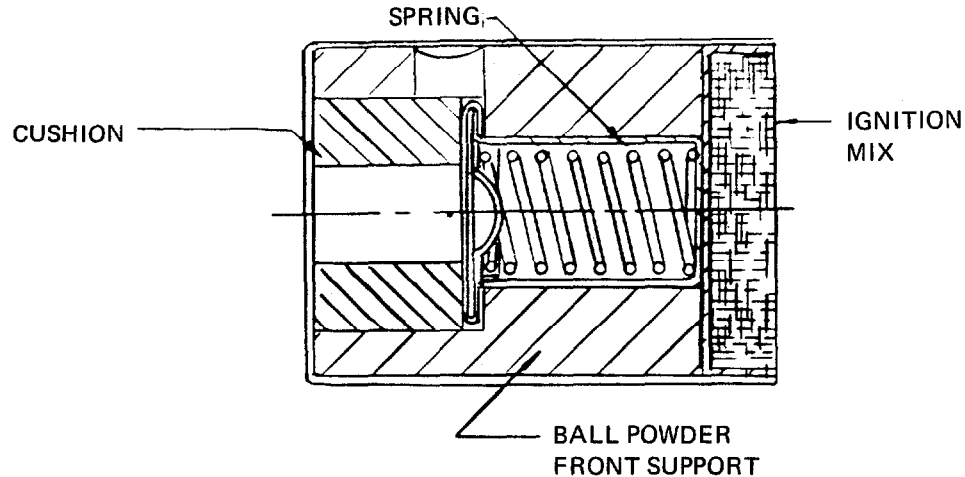
Fig 9 Electrical Ignition Element
